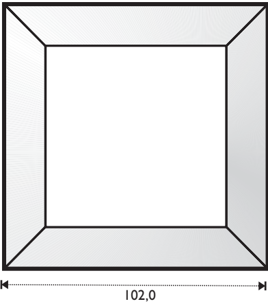
85 341 04 4" x 4"
