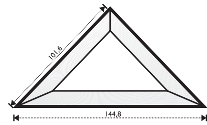
85 380 57 4" x 4" x 5,7"
